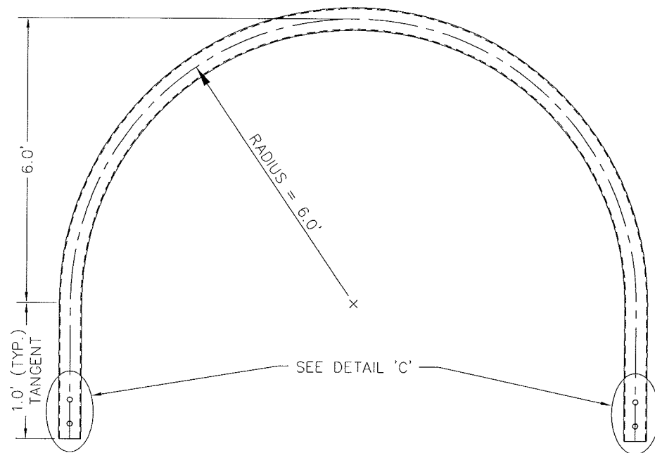
DETAIL 'B'
